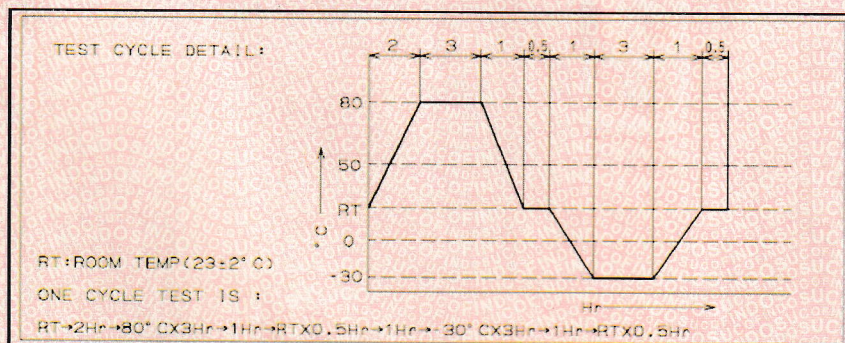
Grafik uji siklus panas (heat cycle test)
